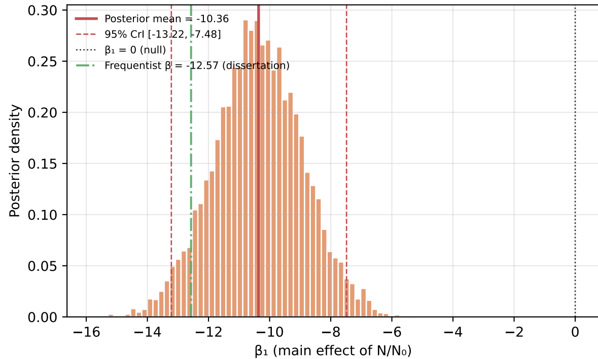
(b) \beta_1 main effect — P(\beta_1 < 0) = 1.000 \Delta\text{AIC} = -72 (B3 vs baseline)
