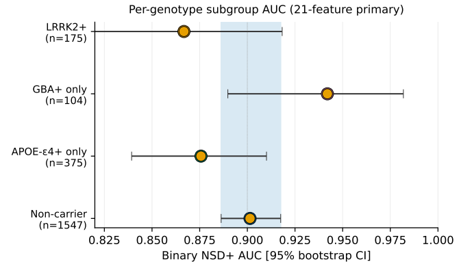
Fig. 8. Subgroup fairness by genetic-carrier status (21-feature primary, binary NSD-ISS). Per-genotype subgroup AUC with 95% bootstrap CIs on the 21-feature strict-circularity primary. Mutually-exclusive carrier strata: LRRK2+ (any), n=175 , AUC 0.867 [0.811, 0.918]; GBA+ only (not LRRK2+), n=104 , AUC 0.942 [0.890, 0.982]; APOE-ε4+ only (not LRRK2+, not GBA+), n=375 , AUC 0.876 [0.839, 0.910]; Non-carrier, n=1,547 , AUC 0.901 [0.886, 0.917]. All four carrier-subgroup CIs overlap the non-carrier reference band (blue shaded), indicating no systematic performance disparity by genetic-carrier status. Top-10 SHAP feature importance (22-feature reference specification) is reported in Supplementary S-2, where the caudate/putamen ratio dominates—the quantitative motivation for its exclusion from the 21-feature primary (§III-D).
