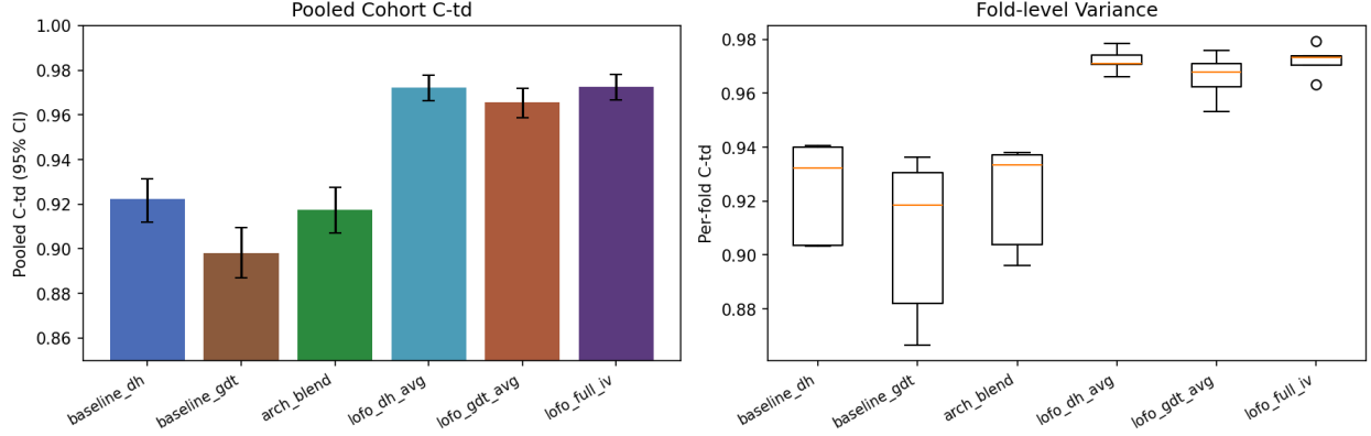
Figure 6: Six-strategy ensemble analysis. Left: pooled cohort C-td (mean \pm 95% bootstrap CI) across six pre-registered strategies; LOFO variants are inflated by CV contamination (asterisk in Table 5). Right: per-fold C-td distributions (boxplot); within-model LOFO ensembling reduces fold-level variance by 72–76%, remediating Graph-DT’s higher single-fold variance. Arch-blend of DeepHit and Graph-DT (third column, left) performs slightly worse than DeepHit alone, supporting a complementarity framing over architectural fusion.
