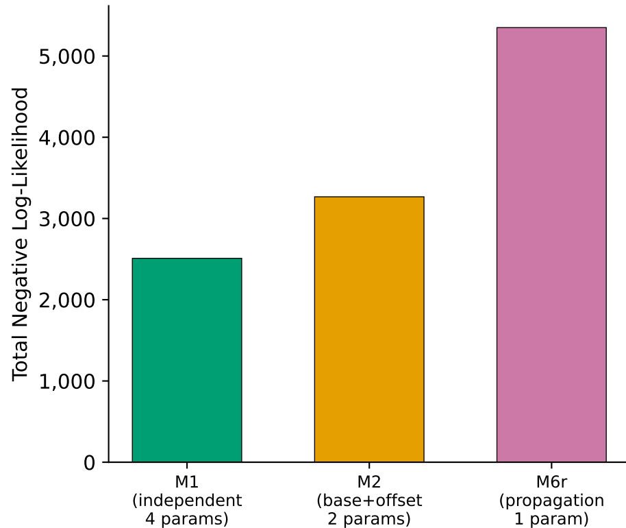
B. Model Comparison: NLL
