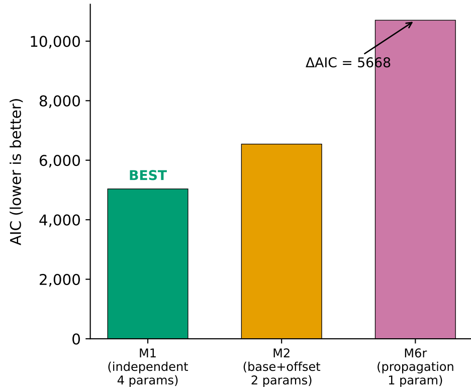
A. Model Comparison: AIC
