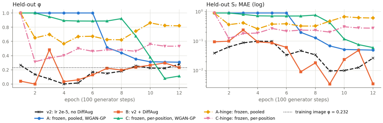
Swin critic probes
