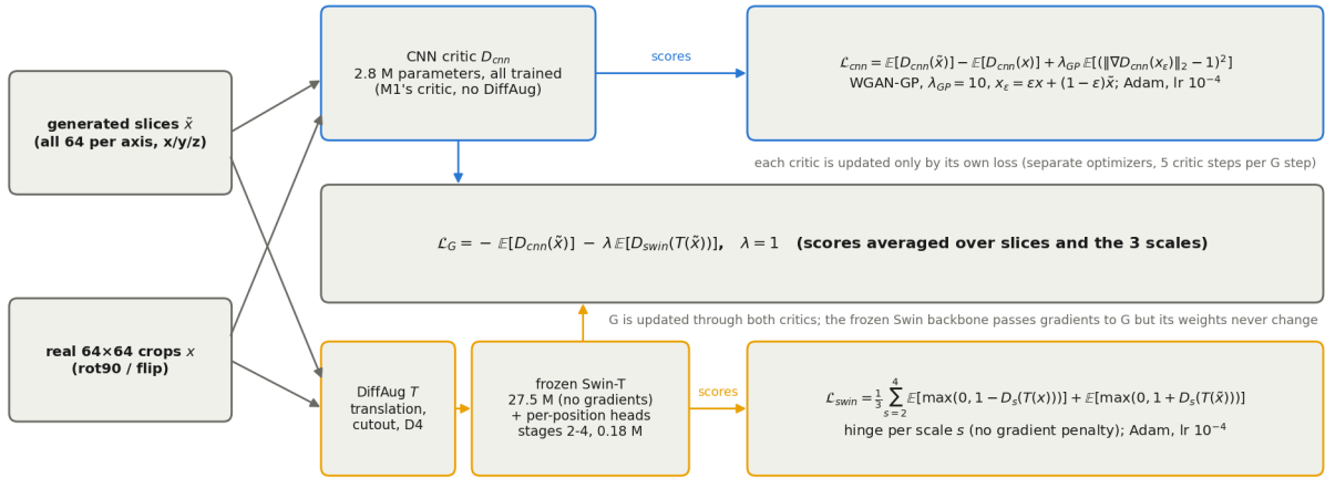
M4 / M5 training objective: CNN critic (WGAN-GP) + frozen Swin-T critic (hinge), summed in the generator loss
