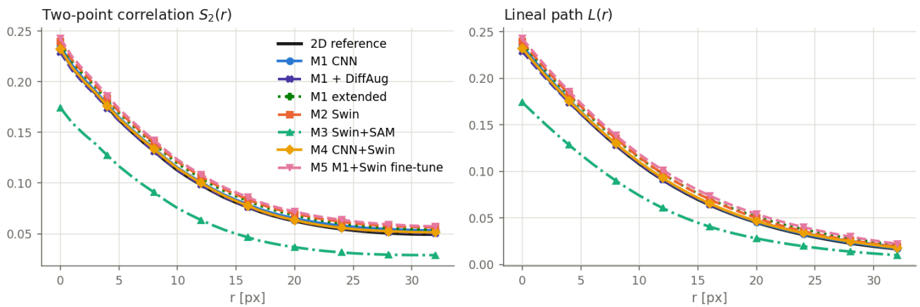
Descriptor curves
