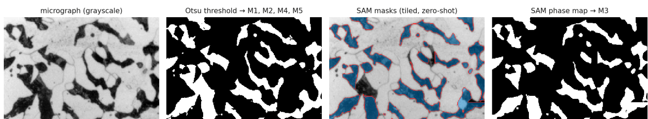
Phase segmentation of MicroLib 000210 (crop): Otsu ( \phi = 0.232 ) vs SAM ( \phi = 0.217 )
