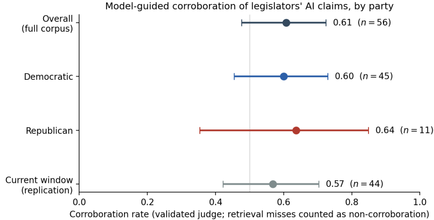
Figure 7: Model-guided corroboration of legislators’ AI claims. The benchmark-validated judge reads the best on-topic reference the model retrieved from the free index for each claim; bars are the corroboration rate with Wilson 95% intervals, counting retrieval misses as non-corroborations. The rate is similar across parties (Democratic 0.60, n=45 ; Republican 0.64, n=11 ) and the current twelve-month window (0.57, n=44 ) reproduces the corpus-wide estimate (0.61). No claim is REFUTED, a property of relevance-seeking retrieval that makes the rate an upper bound on disconfirmation and a lower bound on corroboration.
