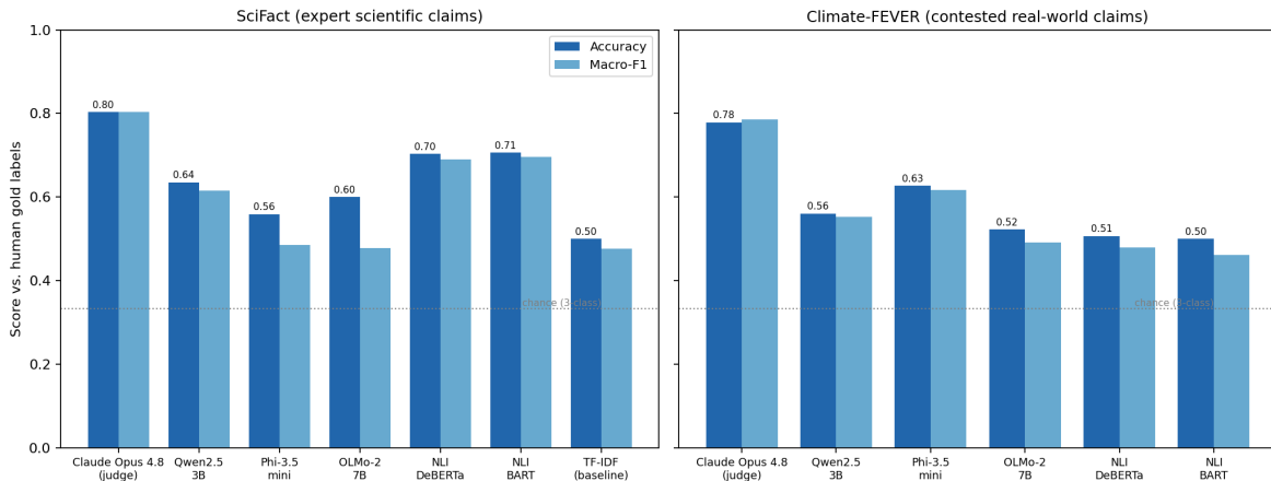
Figure 1: Accuracy and macro- F_1 of each validator against expert-human gold labels, on SciFact (expert scientific claims) and Climate-FEVER (contested real-world claims). The high-capacity LLM judge is the most accurate on both; small open models and zero-shot NLI follow; all exceed chance and the TF-IDF baseline.
