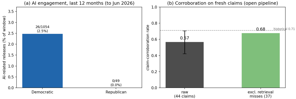
Figure 7: The refreshed pipeline on the most recent twelve months (to June 2026), with no proprietary component anywhere. (a) AI engagement: 26 of 1,054 Democratic releases are AI-related (2.5%) versus 0 of 49 on the sparser Republican caucus site. (b) Corroboration of the 44 freshly extracted empirical AI claims under the fully-open pipeline (model-guided queries \rightarrow free Crossref index \rightarrow benchmark-validated judge): 0.57 raw (Wilson 95% CI shown), 0.68 excluding seven retrieval misses, both near the historical estimate (dashed).
