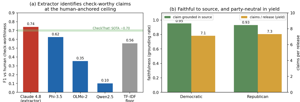
Figure 4: Validating claim extraction with no new human coders. (a) On human-labelled Claim-Buster check-worthiness, the frontier extractor reaches F_1 0.74 (Cohen’s \kappa = 0.53 ), at the Check-That! state-of-the-art band ( \sim 0.70 ); independently-developed models clear the lexical floor. (b) 95% of extracted claims are entailed by (grounded in) their own source release, and extraction yield is party-balanced (7.1 vs 7.3 claims per release).
