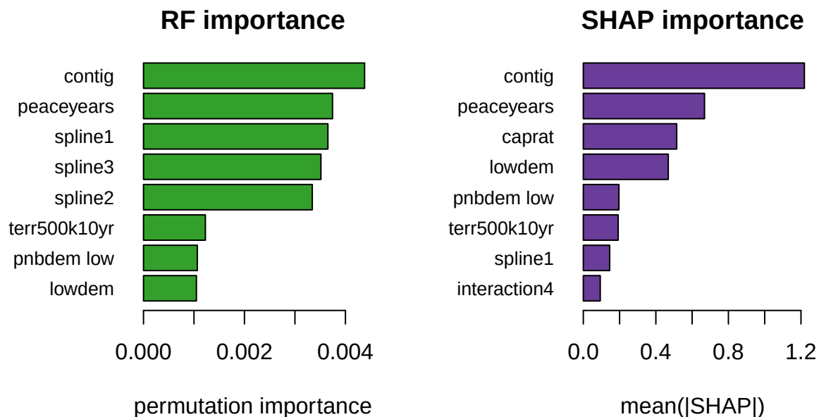
Figure 6: Permutation importance (left) and SHAP importance (right).
