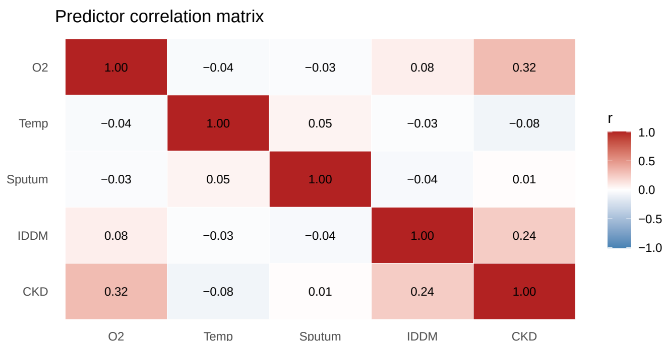
Figure 6: Pairwise Pearson correlations among the five predictors. Correlations are weak; the strongest is O2 with CKD ( r = 0.32 ), well below any collinearity concern.
