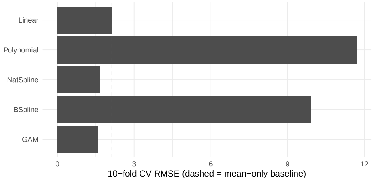
Figure 10: Cross-validated RMSE by mean function. Moving from a straight line to a spline or GAM in firm size lowers held-out error; the extra flexibility of the B-spline/poly is not free once cross-validated.
