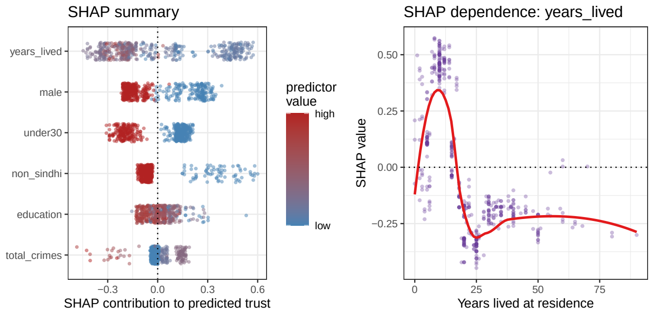
Figure 10: Left: SHAP summary for the xgboost model (training rows); each point is one respondent, x = that predictor's additive contribution to predicted trust, colour = the predictor's value (blue low, red high). Right: SHAP dependence for years lived at residence — the per-respondent contributions trace the same steep-early-drop-then-flatten shape as the partial-dependence curve.
