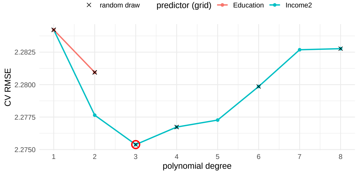
Figure 6: Validation curves from the hyperparameter searches. Grid: CV RMSE vs. polynomial degree for each candidate predictor (lines). Random: sampled configurations (crosses). Both searches converge on the same shallow optimum.
