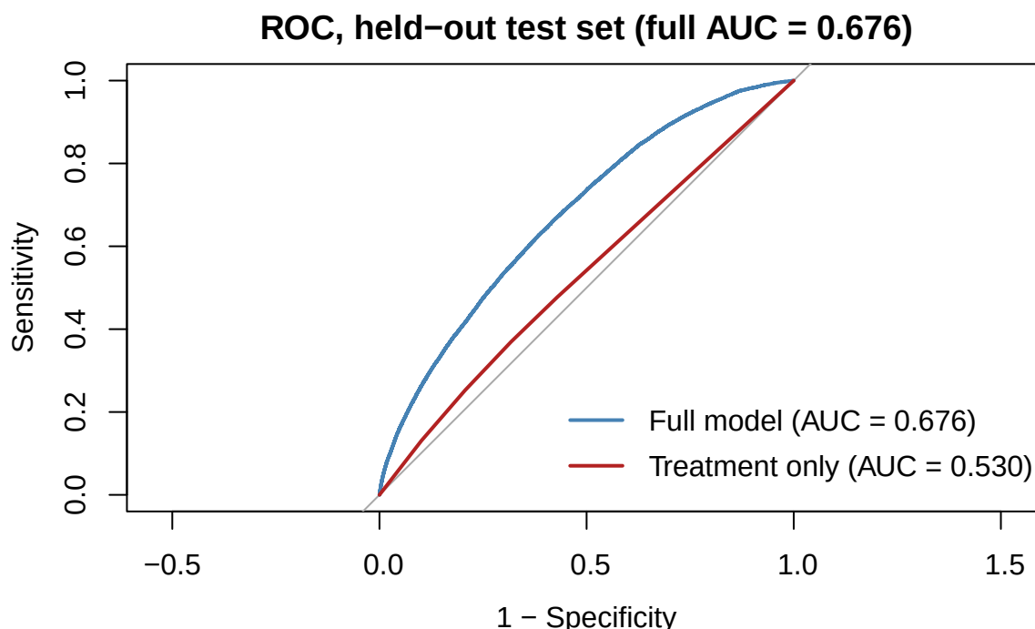
Figure 8: ROC curves on the held-out test set. The full model dominates the treatment-only model everywhere; the treatment-only curve hugs the diagonal, showing that experimental assignment alone barely ranks voters above non-voters.
