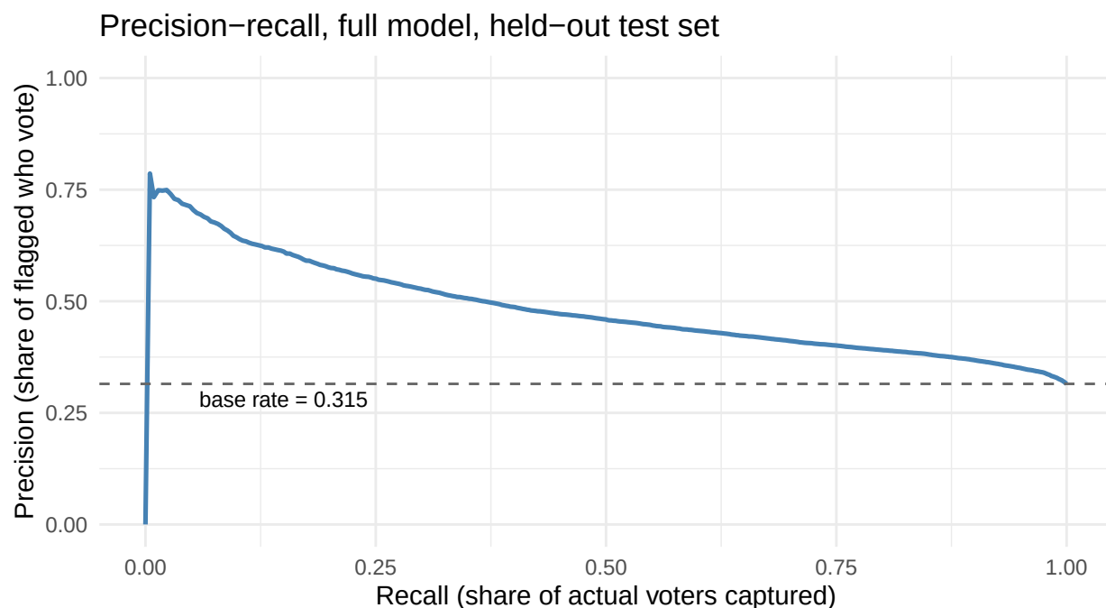
Figure 9: Precision-recall on the held-out test set. The dashed line is the base rate (~32 percent), the precision of flagging everyone. The full model reaches roughly 80 percent precision on its most confident picks and degrades gracefully toward the base rate as recall approaches 1.
