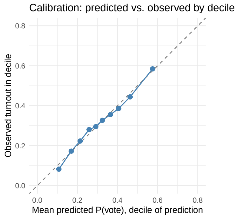
Figure 10: Reliability curve on the held-out test set: mean predicted probability vs. observed turnout within deciles of the prediction. Points sit on the 45-degree line across the whole range – the logit’s probabilities mean what they say.
