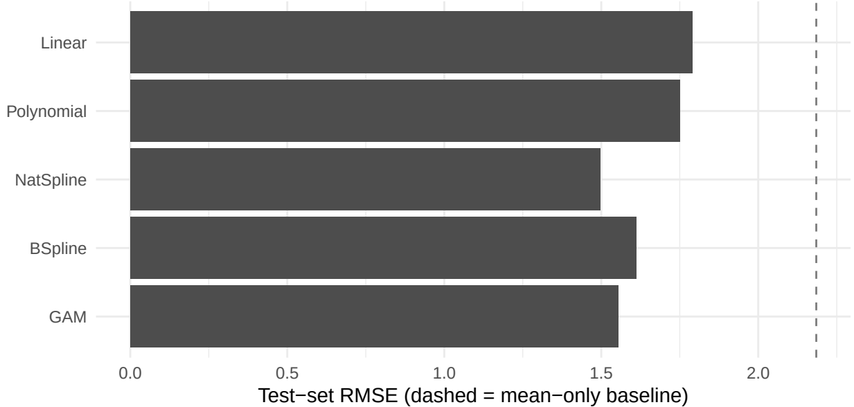
Figure 10: Held-out test-set RMSE by mean function (dashed = mean-only baseline). Global unpenalized bases (cubic polynomial, high-df B-spline) can extrapolate wildly at test firms outside the training range of firm size.
