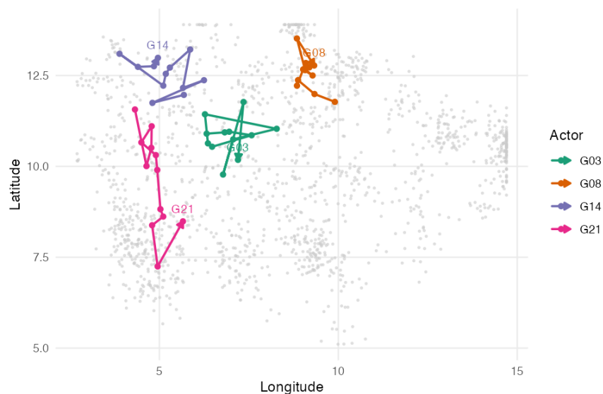
Figure 1: Projected locations of four actors in the simulated nigeria_sim data, fit with the one-parameter model and projected at yearly intervals from 2005 to 2016. Grey points are the observed dyadic events; coloured paths trace each actor's PALS-projected trajectory (arrows point forward in time).
