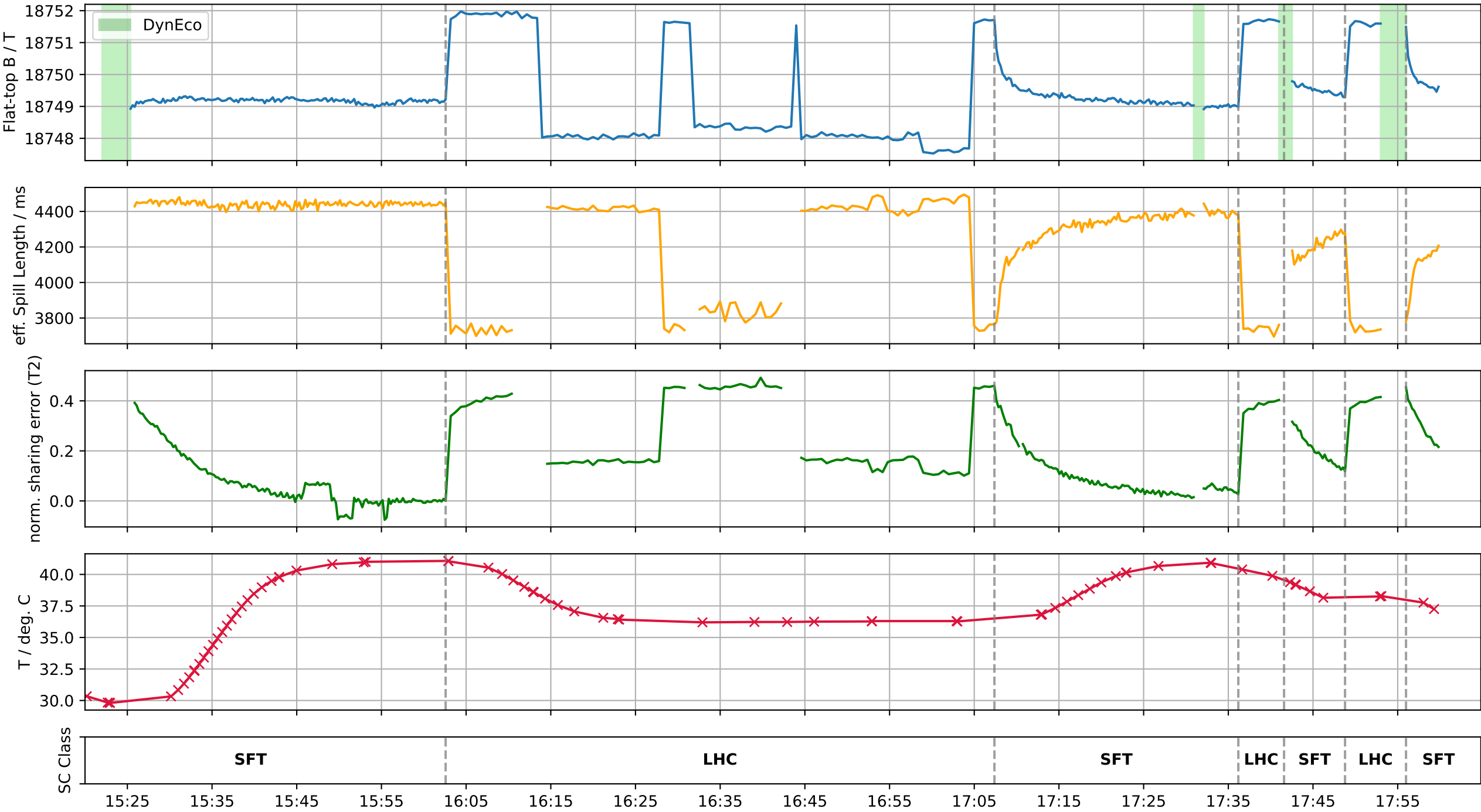
Evolution of SFTPRO1 flat-top parameters during 06-05-2026 MD
