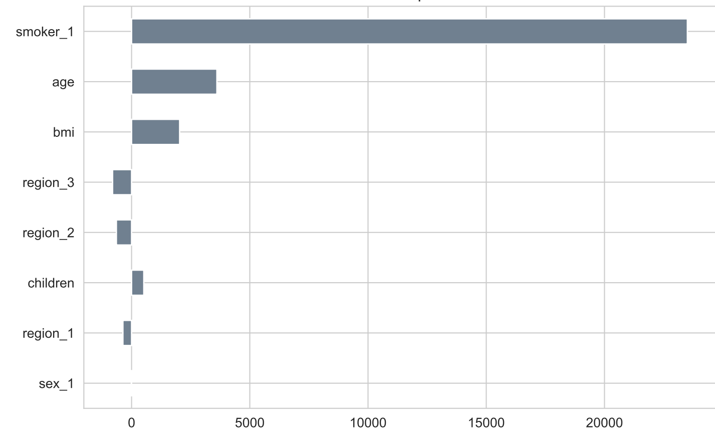
Coefficient Importance
