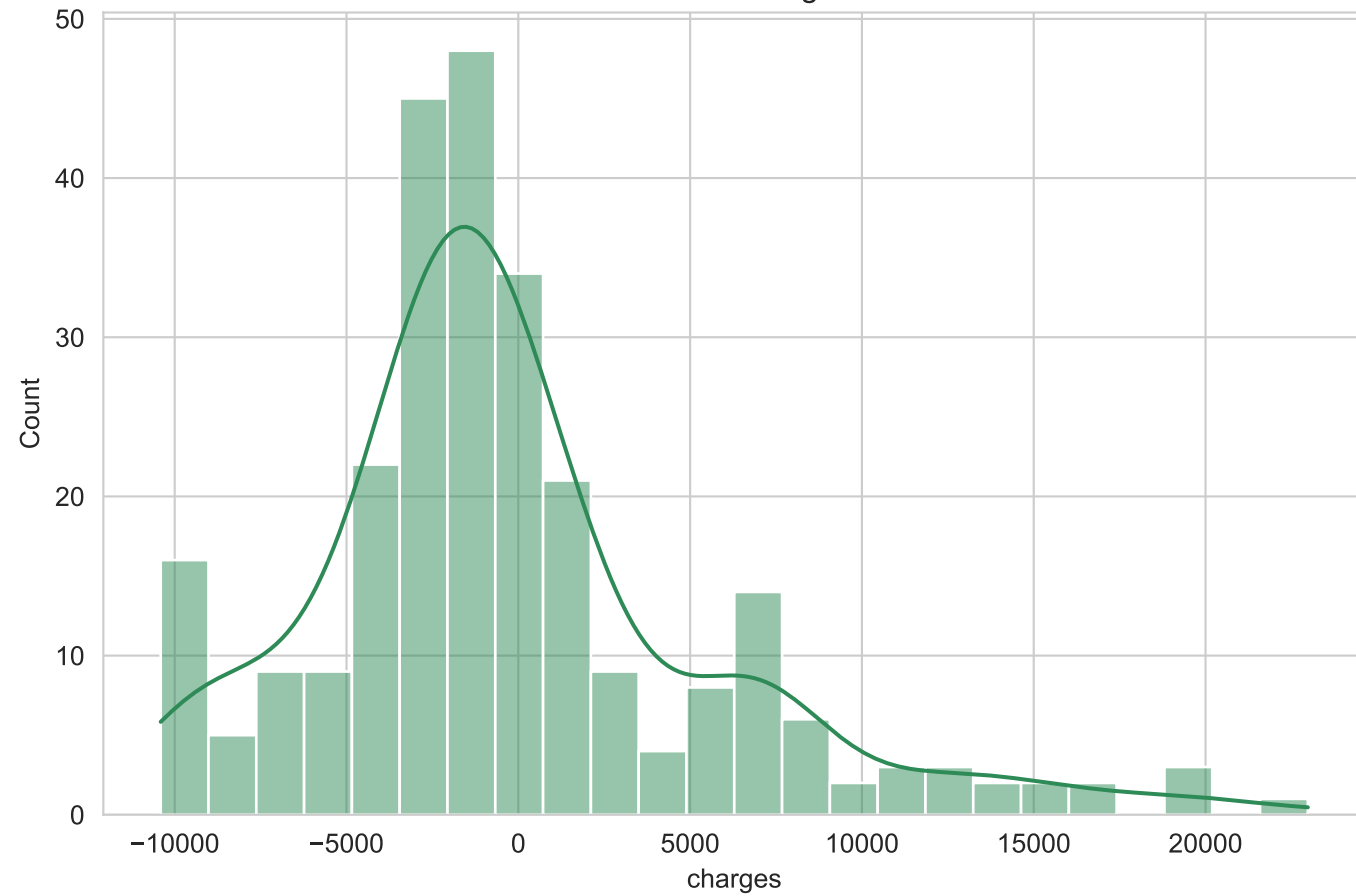
Residual Histogram
