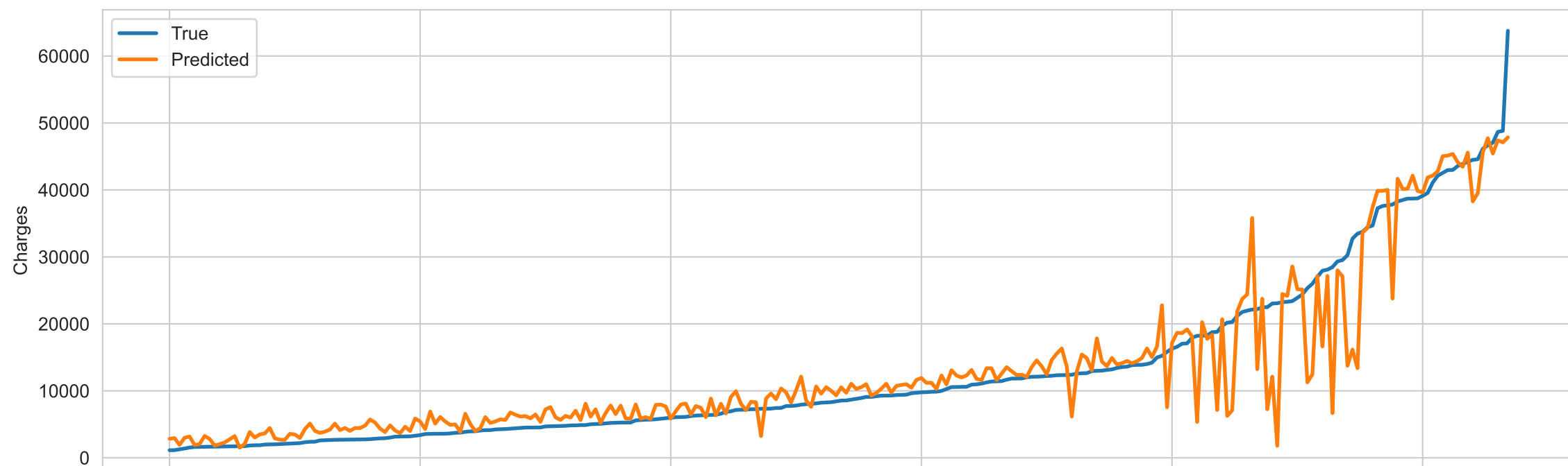
Hist GBR
