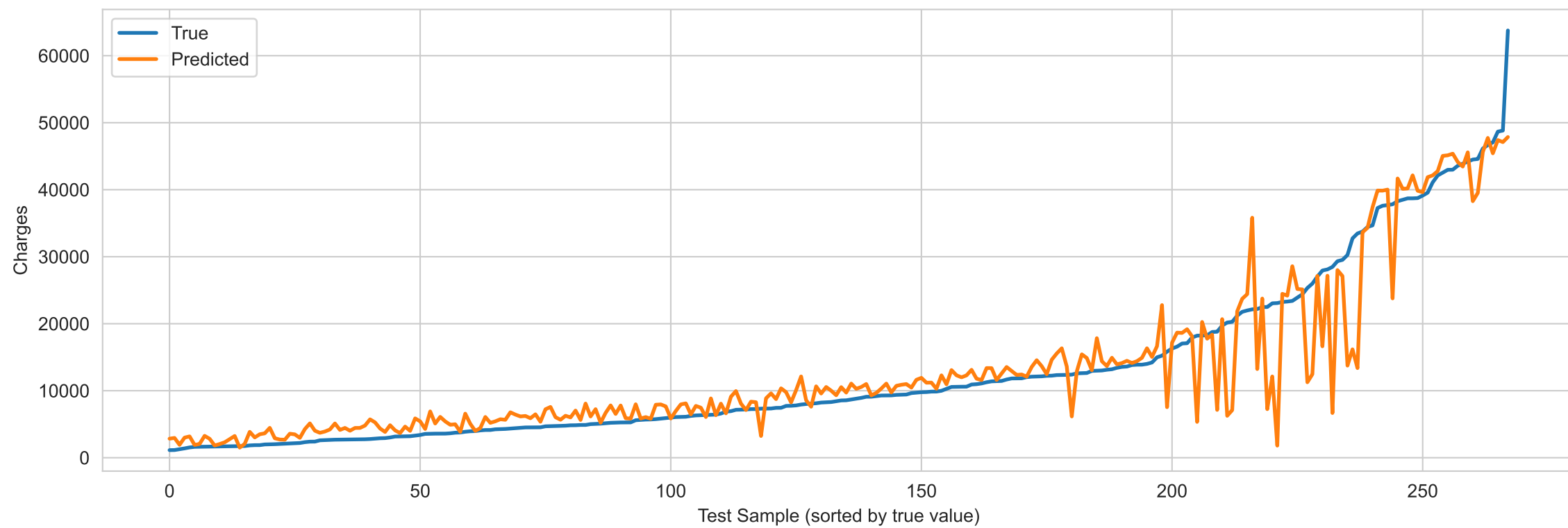
Tuned GBR
