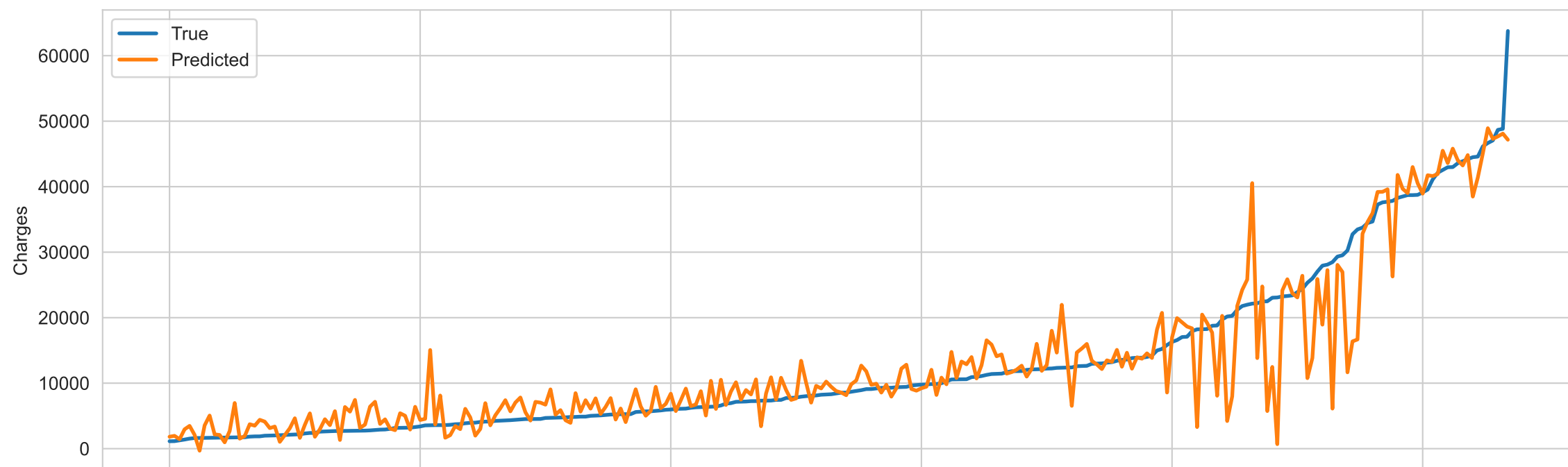
Tuned GBR
