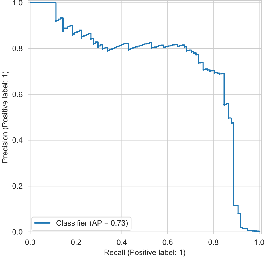
Precision-Recall Curve
