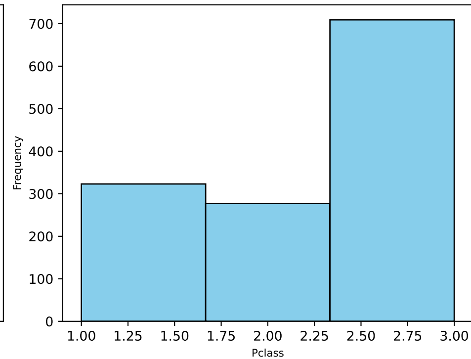
Distribution of Pclass
