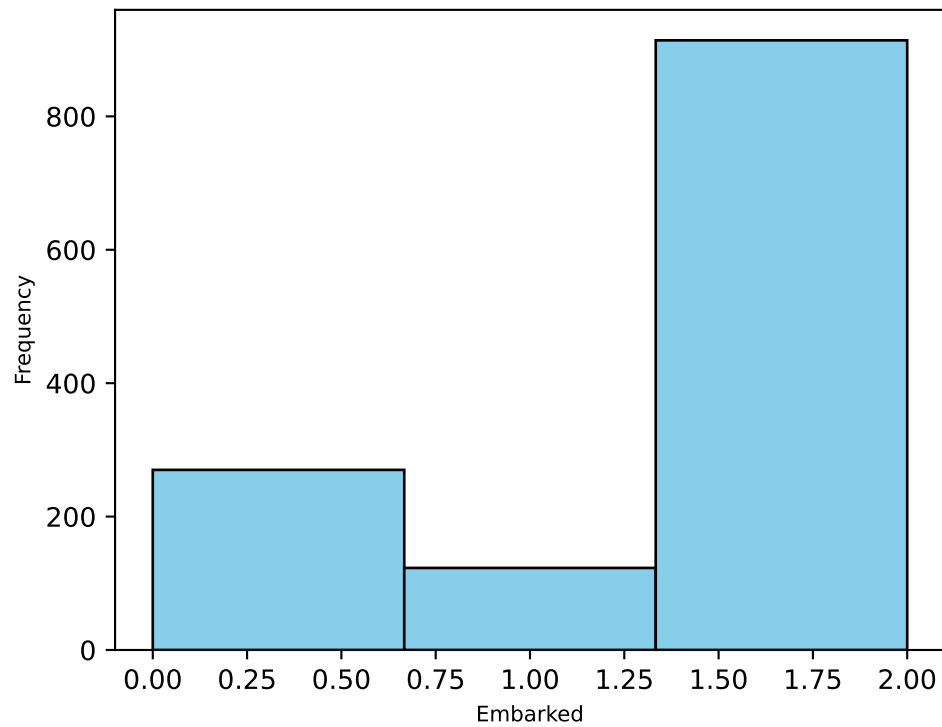
Distribution of Embarked
