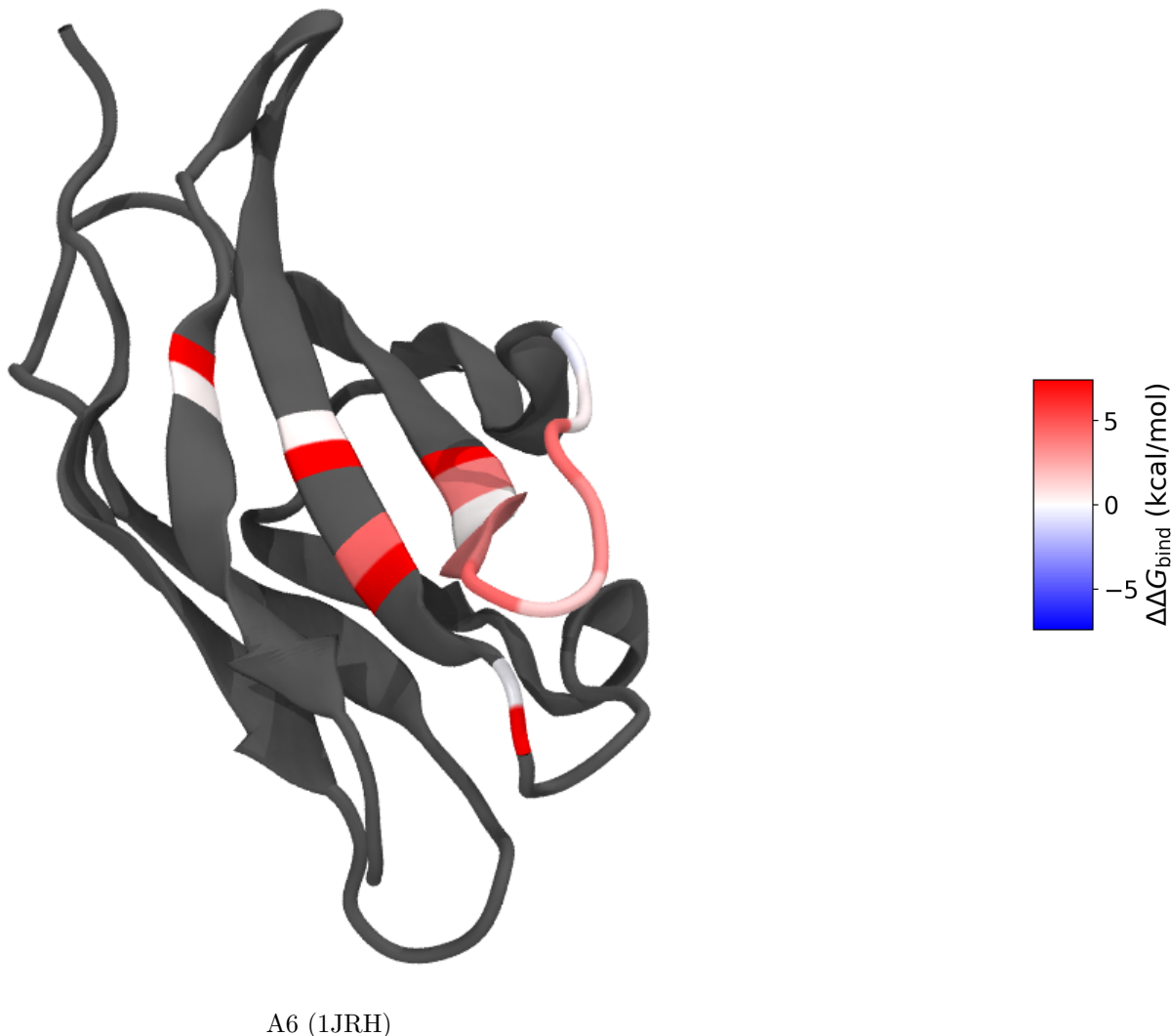
Figure 7: IFN- \gamma receptor coloured per residue by A6 alanine-scan \Delta\Delta G_{\text{bind}} (shared scale, white = 0, red = hotspot; grey = not scanned). The hotspots cluster on a single \beta -sandwich face.
