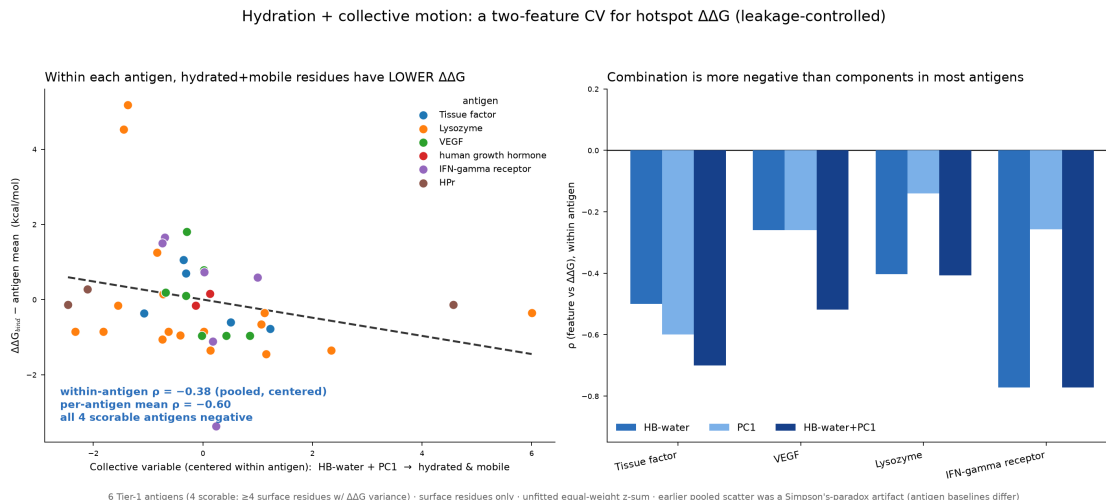
Figure 18: Hydration + collective motion. The equal-weight, unfitted collective variable z(\text{HB}_{\text{water}}) + z(P^{(1)}) vs. \Delta\Delta G_{\text{bind}} , centred within antigen so the pooled slope matches the per-antigen effect (per-antigen \rho = -0.60 ); the pooled uncentred cloud inverts by Simpson's paradox and is not the honest view. Right: within-antigen \rho for the combination against its two components. analysis/combined_cv.py .
