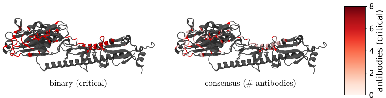
Figure 12: Influenza hemagglutinin (H3 X-31, 1HGG protomer) : 84 wild-type-verified critical residues (HA1 head + HA2 stem) from 79 antibodies, binary and antibody-frequency consensus. Critical residues concentrate on the HA1 globular head (the classic antigenic sites) with a sparser stem contribution. Native HA is an obligate trimer; one protomer is shown.
