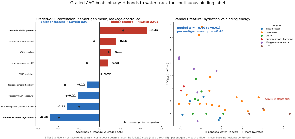
Figure 17: Grading the label beats thresholding it. Per-antigen Spearman \rho of each feature against continuous \Delta\Delta G_{\text{bind}} (surface residues; pooled \rho overlaid as points). Hydration leads; interaction energy — the binary winner — is flat on the gradient. Right: the water-H-bond vs. \Delta\Delta G_{\text{bind}} relation, coloured by antigen. analysis/graded_ddg.py .
