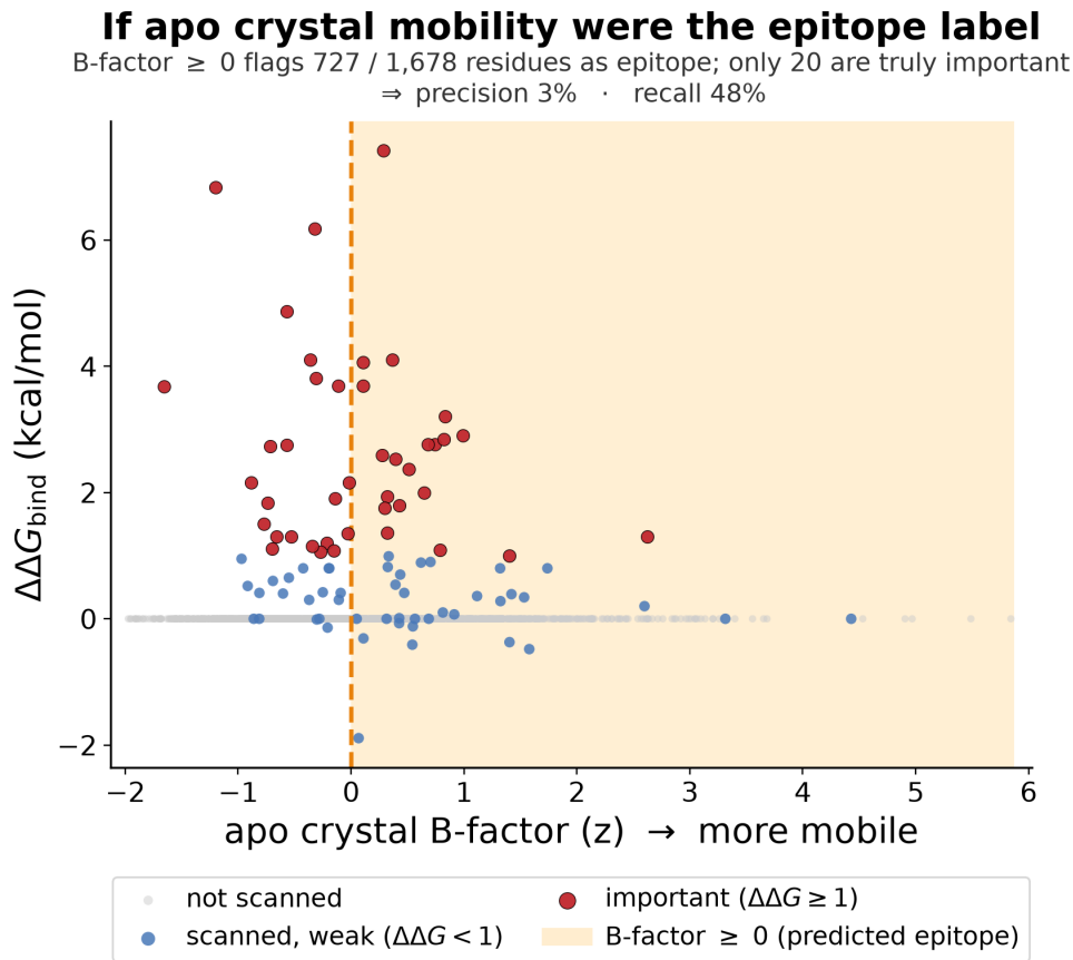
Figure 14: Crystallographic mobility as an epitope label (apo structures). Per-residue C \alpha B-factor (z-scored per structure; right = more mobile) on genuine apo (antibody-free) crystals vs. alanine-scan \Delta\Delta G_{\text{bind}} , colours as in Fig. 13. The important (red) residues lean toward low B-factor (rigid) rather than the high-mobility band, but only weakly (pooled Spearman -0.23 ; -0.29 on the complex-bound set) and inconsistently across antigens. analysis/recompute_apo_baselines.py + plot_feature_vs_label.py .
