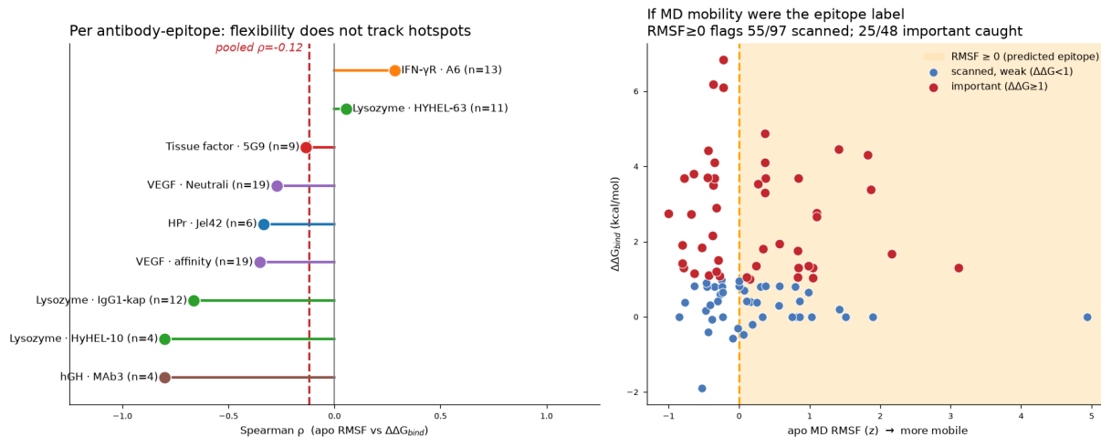
Figure 15: Apo-MD flexibility as an epitope label. Left: Spearman \rho between per-residue apo RMSF and alanine-scan \Delta\Delta G_{\text{bind}} for each antibody-epitope (coloured by antigen; dashed line is the pooled value); the correlations scatter around zero with a slight negative lean. Right: all 97 scanned residues, RMSF ( z ; right = more mobile) vs. \Delta\Delta G_{\text{bind}} , colours as in Fig. 14 — the important (red) residues are spread across the mobility range, not concentrated on the mobile side. An \text{RMSF} \geq 0 cutoff (the shaded band) flags 55 of 97 scanned residues and catches 25 of 48 hotspots — no better than a coin toss on this set. analysis/rmsf_dynamics_baseline.py . MT-SP1 (no apo MD) and Dengue E (10KE, Tier-2) are not in this graded set; HA (1HGG) pending.
