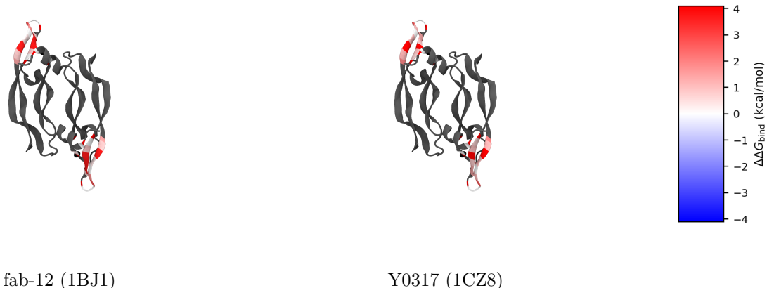
Figure 3: VEGF-A homodimer coloured per residue by \Delta\Delta G_{\text{bind}} for each antibody (shared scale, white = 0; grey = not scanned). Both protomers carry the same labelled residues; red marks the hotspots.
