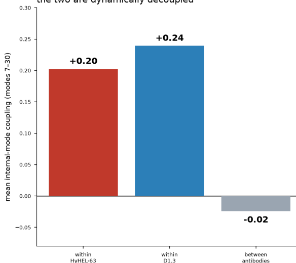
Figure 20: Two antibodies, two dynamically distinct patches. Leave-one-antibody-out on lysozyme: HyHEL-63 and D1.3 footprints each co-move internally and are decoupled from one another ( -0.02 ). The patches are real per-antibody footprints, not a pooling artefact — but see Fig. 21. analysis/freesean_involvement.py .
