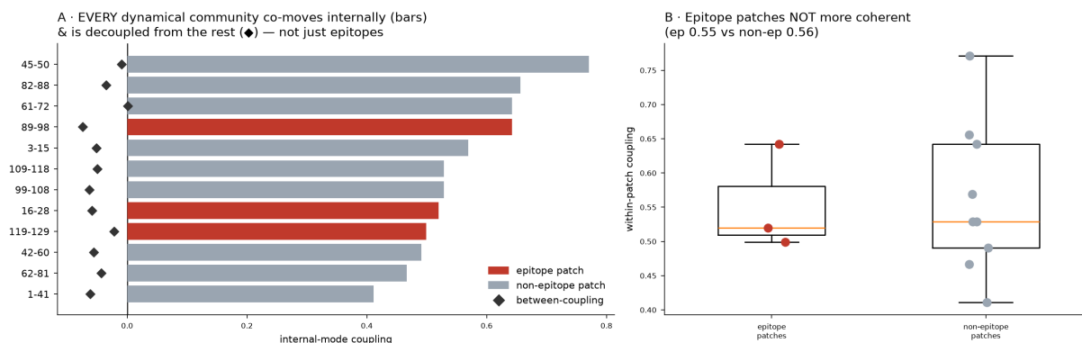
Figure 21: The decoupled-patch property is generic. All 12 dynamical communities of 1AKI co-move internally (bars) and decouple from the rest (◆); epitope patches (red) are no more coherent than non-epitope patches (grey). analysis/freesean_involvement.py .
