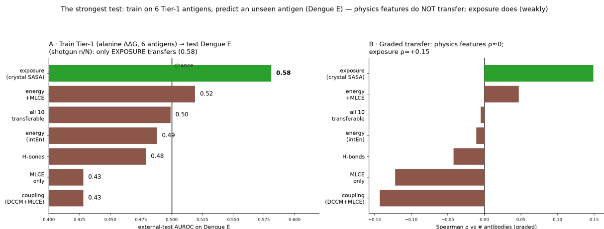
Figure 23: The strict test: train Tier-1, predict Dengue E. Physics-feature sets (energy, H-bonds, dynamical and energetic coupling) all transfer at chance to an unseen antigen and a different label type; only exposure transfers (0.58, \rho = +0.15 ). analysis/external_dengue.py .
