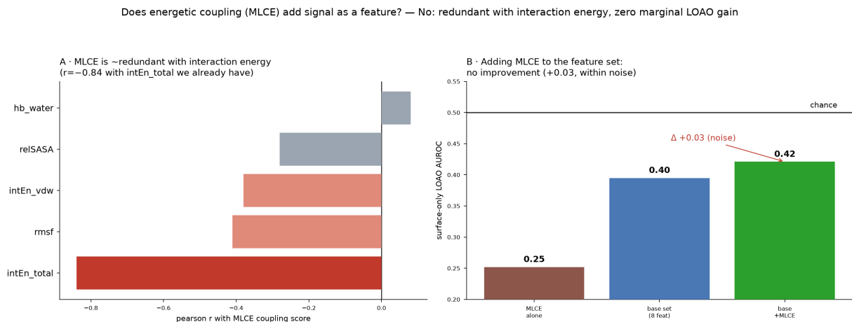
Figure 22: MLCE energetic coupling adds nothing as a feature. Left: the MLCE score is largely redundant with per-residue interaction energy ( r = -0.84 ). Right: adding it to the 8-feature surface LOAO model yields +0.03, within noise. analysis/mlce.py .
