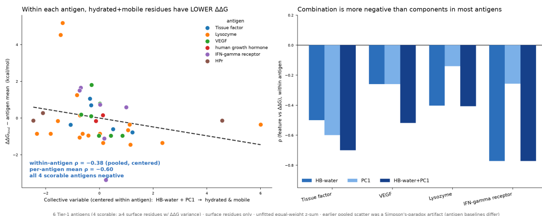
Figure 18: Hydration + collective motion. The equal-weight, unfitted collective variable z(\text{HB}_{\text{water}}) + z(P^{(1)}) vs. \Delta\Delta G_{\text{bind}} , centred within antigen so the pooled slope matches the per-antigen effect (per-antigen \rho = -0.60 ); the pooled uncentred cloud inverts by Simpson’s paradox and is not the honest view. Right: within-antigen \rho for the combination against its two components. analysis/combined_cv.py .
