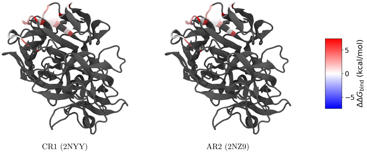
Figure 5: Bont/A1 H C coloured per residue by \Delta\Delta G_{\text{bind}} for two neutralizing mAbs (shared scale, white = 0; grey = not scanned). Red marks the hotspots — the strongest reach \Delta\Delta G_{\text{bind}} > 7 (binding essentially abolished).
