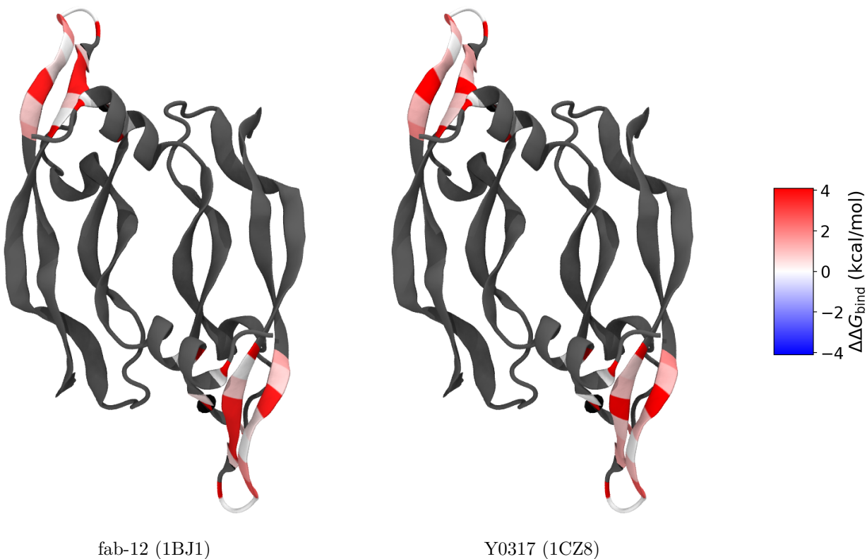
Figure 3: VEGF-A homodimer coloured per residue by \Delta\Delta G_{\text{bind}} for each antibody (shared scale, white = 0; grey = not scanned). Both protomers carry the same labelled residues; red marks the hotspots.
