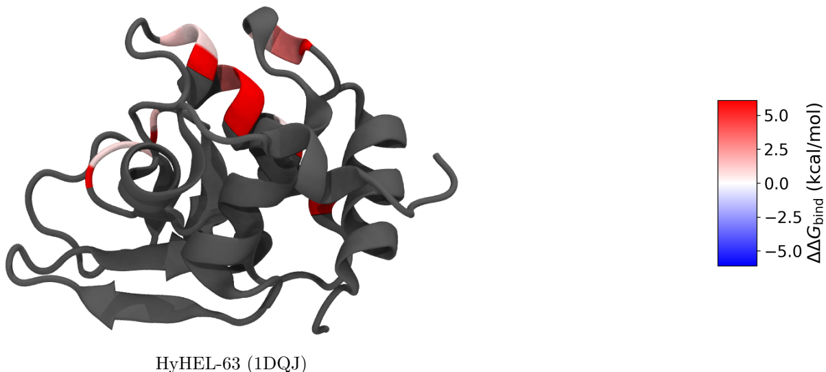
Figure 1: HEL coloured per residue by HyHEL-63 alanine-scan \Delta\Delta G_{\text{bind}} (white = 0, red = hotspot, blue < 0; grey = not scanned). Red marks the candidate epitope core.
