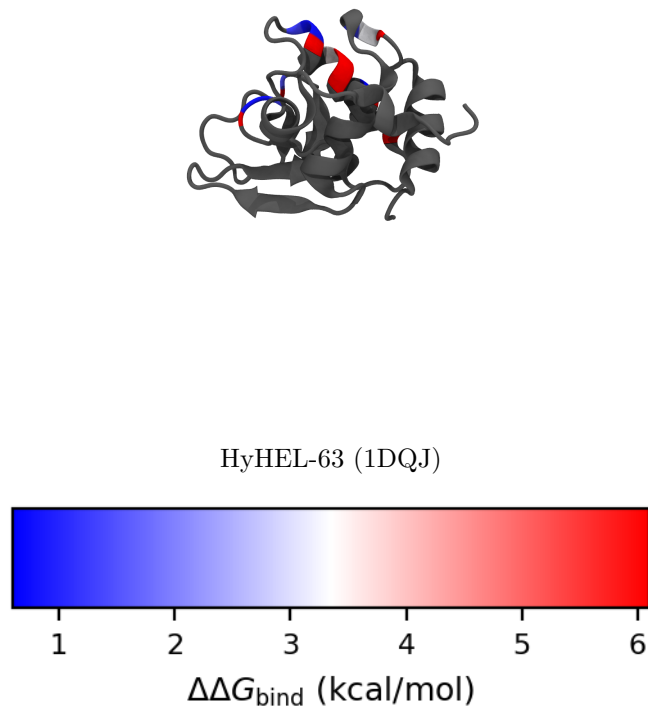
Figure 1: HEL coloured per residue by HyHEL-63 alanine-scan \Delta\Delta G_{\text{bind}} (grey = residue not scanned). Red marks the energetic hotspots — candidate epitope core.
