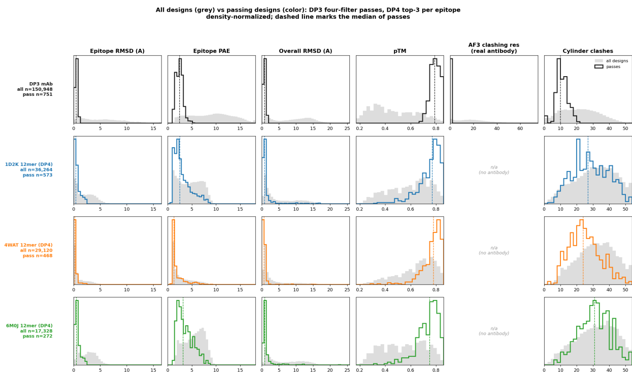
Figure 7: All designs (grey) versus passing designs (colored outline), per metric and per row. DP3 passes are the four-filter set; DP4 passes are the top 3 per epitope by composite score. Dashed lines mark the median of the passing set. Regenerated by episcaf_analysis/viz/plot_passes_overlay.py .
