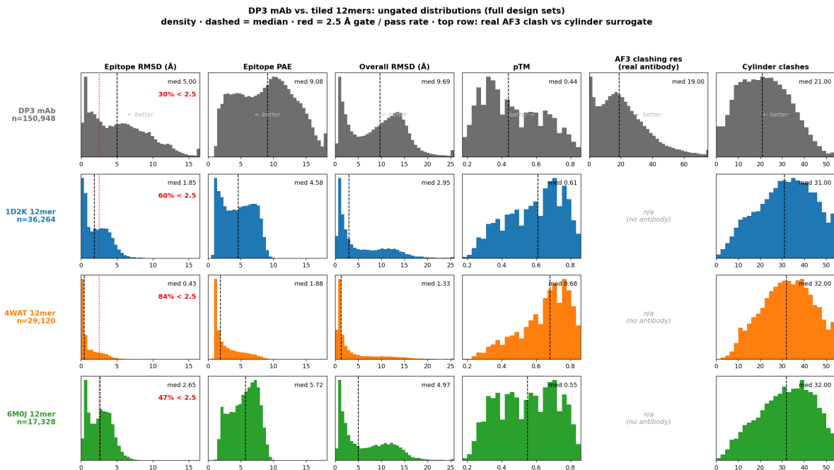
Figure 3: Ungated metric distributions (full design sets), DP3 mAb versus the three 12-mer antigens, across epitope RMSD, epitope PAE, overall RMSD, pTM, AF3 clashing residues (antibody set only), and cylinder clashes. Dashed line marks the median; red marks the 2.5 Å epitope-RMSD gate with the per-set pass rate. Regenerated by notebooks/dp3_vs_12mer_distributions.ipynb .
