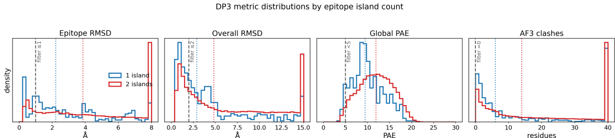
Figure 8: DP3 design metrics (RFD1+MPNN, dp2.parquet ) split by epitope island count: blue = single-island ( n = 549 ), red = two-island ( n = 123813 ); only designs with an AF3 result are included. Panels, left to right: epitope-chunk RMSD, overall RMSD, global mean PAE, and number of AF3 clashing residues, the four selection metrics. Distributions are area-normalized (density) because the groups differ in size by \sim 200\times . Dotted vertical lines mark each group’s median; dashed grey lines mark the four-filter thresholds (epitope RMSD \leq 1 , overall RMSD \leq 2 , PAE < 5 , clashes = 0). Single-island designs are shifted toward better values on every metric (median epitope RMSD 2.22 vs 3.86 Å, median PAE 9.5 vs 11.9). Regenerated by episcaf_analysis/viz/plot_island_split.py .
