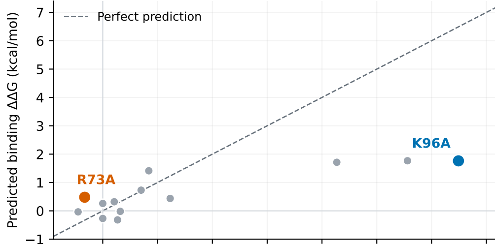
Lennard-Jones only · 201 frames n = 13; Spearman \rho = +0.73
