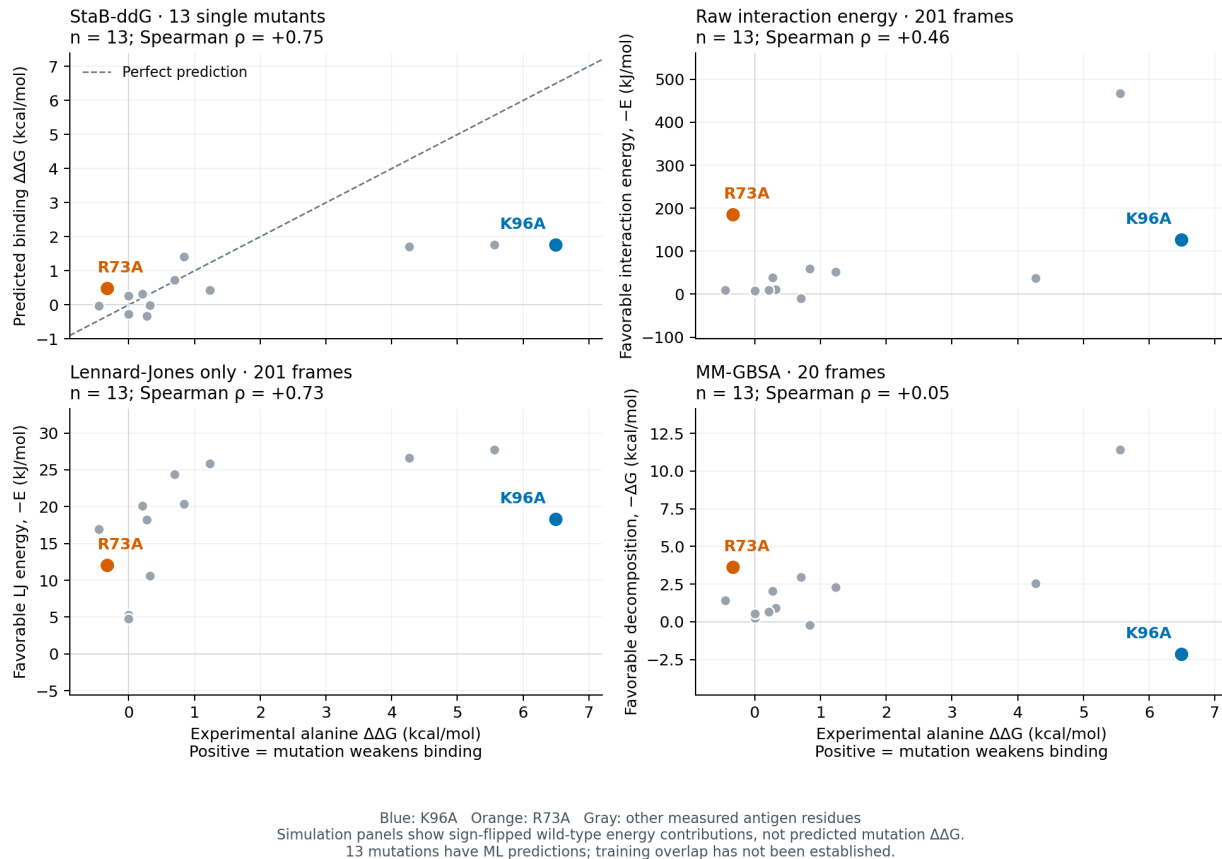
Figure 3: The learned predictor and simulation signals against experimental antigen alanine \Delta\Delta G . Blue and orange identify K96A and R73A in every panel. Every panel includes the same thirteen measured antigen residues, with ML values from the full scan. The identity line applies only to predicted mutational \Delta\Delta G . Simulation energies are sign-flipped so more favorable contributions point upward, with their own units and independent vertical scales. Rank correlations use all thirteen measured residues; the earlier two-point pilot is retained separately and not pooled. Generated by energetics/tamarind/plot_comparison.py ; plotted values are saved as a CSV.
