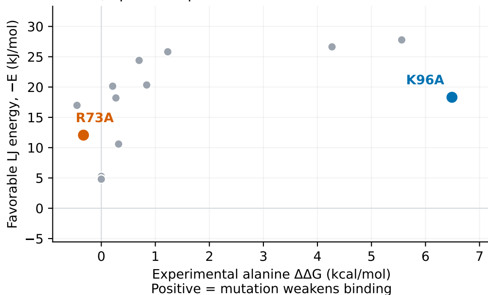
Lennard-Jones only · 201 frames n = 13; Spearman \rho = +0.73
