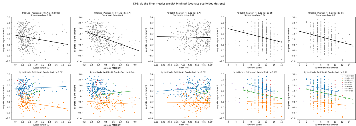
Figure 10: Each metric versus cognate log-enrichment. Top row pooled (one trend line); bottom row colored by antibody with per-antibody trend lines and the within-antibody fixed-effect correlation in the title. Epitope RMSD’s strong pooled slope (column 2) flattens once colored by antibody — the pooled line was riding the gap between the high-binding 7ox3 band and the low-binding 5fhx band. The native-aware cylinder (right column) slopes down both pooled and within every antibody: more scaffold mass blocking the antibody approach, less binding.
