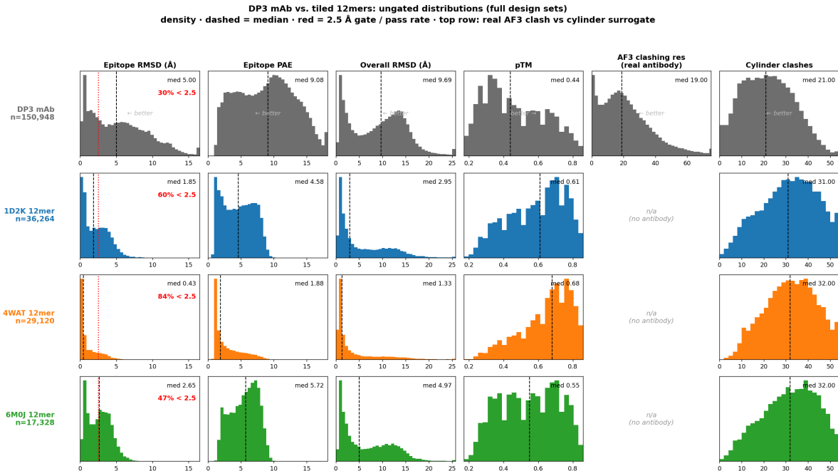
Figure 3: Ungated metric distributions (full design sets), DP3 mAb versus the three 12-mer antigens, across epitope RMSD, epitope PAE, overall RMSD, pTM, AF3 clashing residues (antibody set only), and cylinder clashes. Dashed line marks the median; red marks the 2.5 Å epitope-RMSD gate with the per-set pass rate. Regenerated by notebooks/dp3_vs_12mer_distributions.ipynb .
