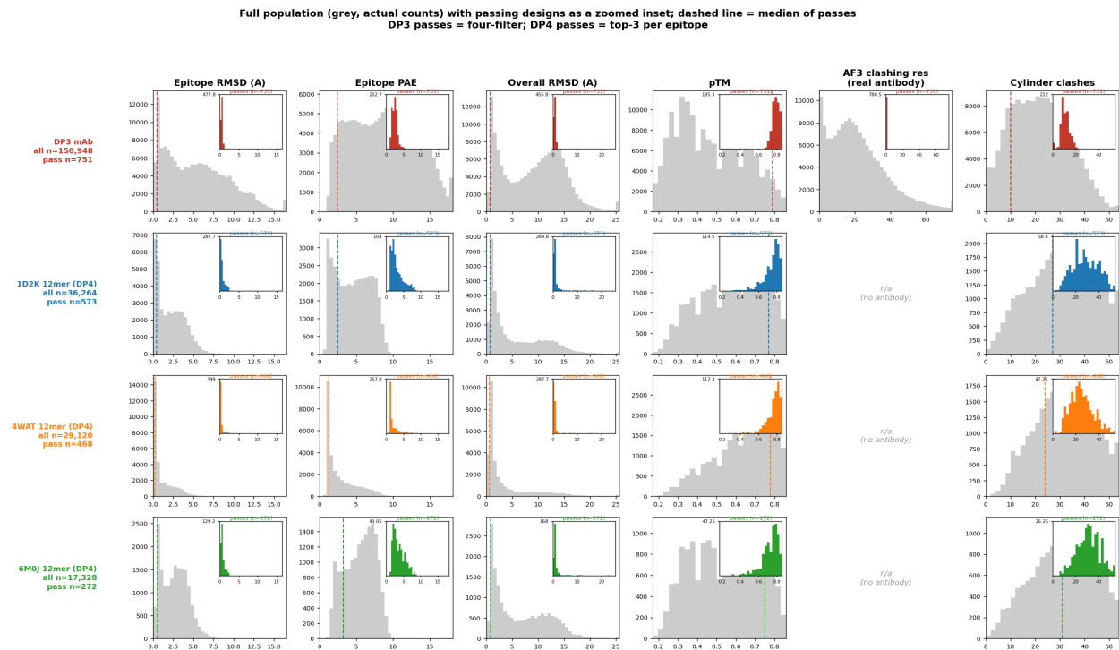
Figure 7: Full design population in actual counts (grey), per metric and per row, with a dashed line marking the median of the passing designs and a zoomed inset showing the passing distribution's own shape and count. Counts (not density) make clear how small and where the selected slice sits; the inset recovers the accepted shape, which is otherwise invisible next to the full population. DP3 passes are the four-filter set; DP4 passes are the top 3 per epitope by composite score. Regenerated by episcaf_analysis/viz/plot_passes_overlay.py .
