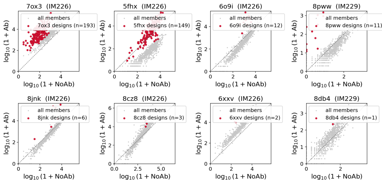
Figure 8: DP3 binding, one panel per antibody: \log_{10}(1 + \text{NoAb}) (x) versus \log_{10}(1 + \text{Ab}) (y), all 1000 library members in grey, the cognate scaffolded designs in red, dashed line y = x . The two well-sampled antibodies (7ox3, n = 193 ; 5fhx, n = 149 ) put the bulk of their designs clearly above the diagonal; the small- n antibodies show a handful of points each, mostly above the line. Panels are on independent axes because absolute counts are not comparable across antibodies/runs.
