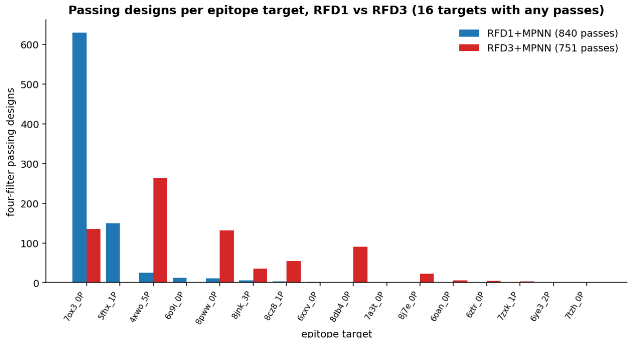
Figure 2: Four-filter passing designs per epitope target, RFD1+MPNN (blue) versus RFD3+MPNN (red). RFD1 is dominated by 7ox3_0p; RFD3 distributes passes across more targets. Regenerated by episcaf_analysis/viz/plot_passes_per_epitope.py .
