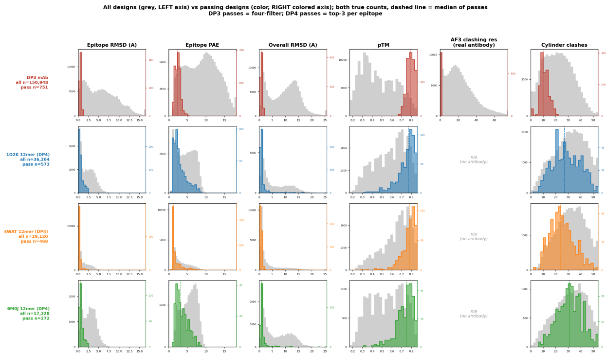
Figure 7: All designs (grey, left axis) and passing designs (color, right colored axis), both in true counts, per metric and per row; the dashed line marks the median of the passes. The twin axes keep the full population and the much smaller passing set each at its own scale, so the shape of the accepted distribution and where it lands are both visible. DP3 passes are the four-filter set; DP4 passes are the top 3 per epitope by composite score. Regenerated by episcaf_analysis/viz/plot_passes_overlay.py .
