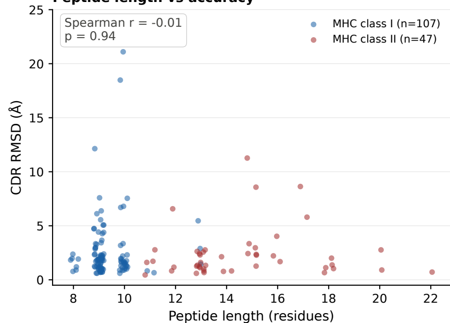
Peptide length vs accuracy
