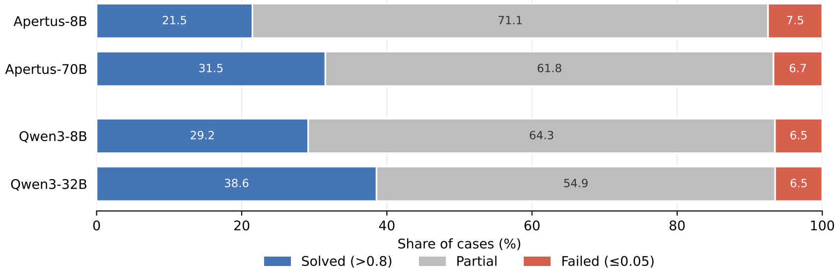
ConGra no-skill baseline: solved / partial / failed (python-tiny, max(edit, winnowing))
