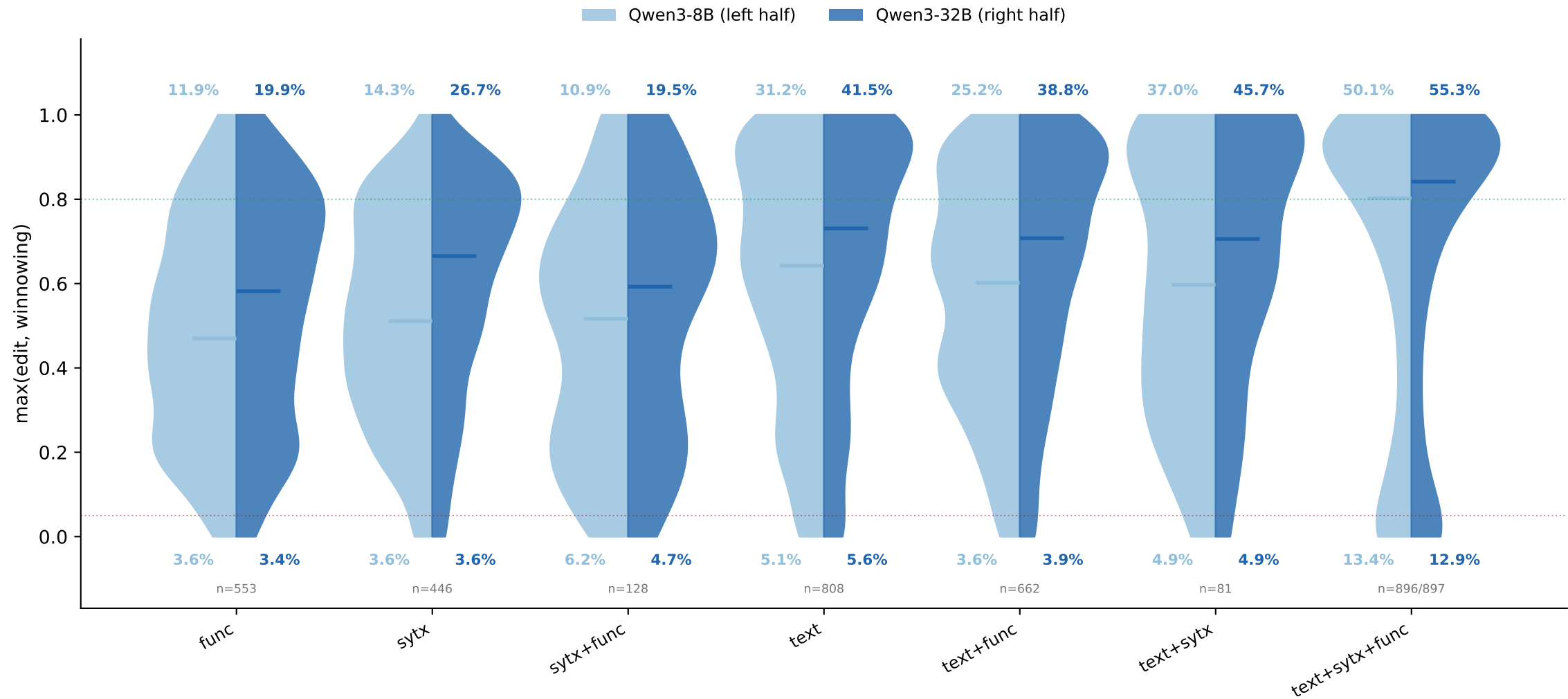
Qwen3 baseline scaling — Qwen3-8B (left half) vs Qwen3-32B (right half) per bucket (no-skill, python-tiny) solved % above ( >0.8 ); failed % below ( \leq 0.05 ); colour-coded median line per model
