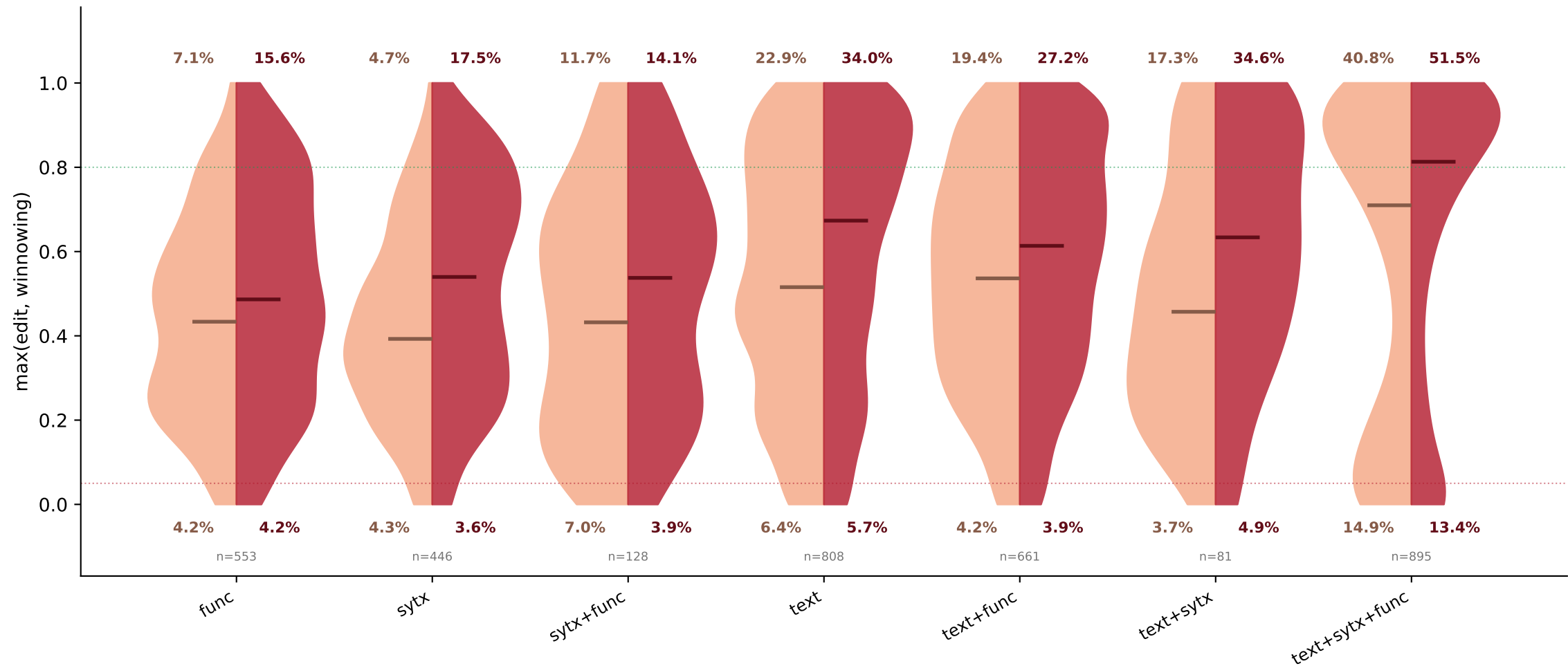
Apertus baseline scaling — Apertus-8B (left half) vs Apertus-70B (right half) per bucket (no-skill, python-tiny) solved % above ( >0.8 ); failed % below ( \leq 0.05 ); colour-coded median line per model
