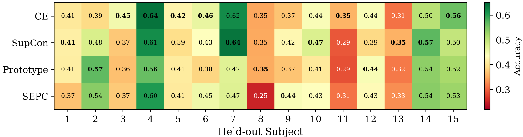
Best Val Accuracy by Method and Subject
