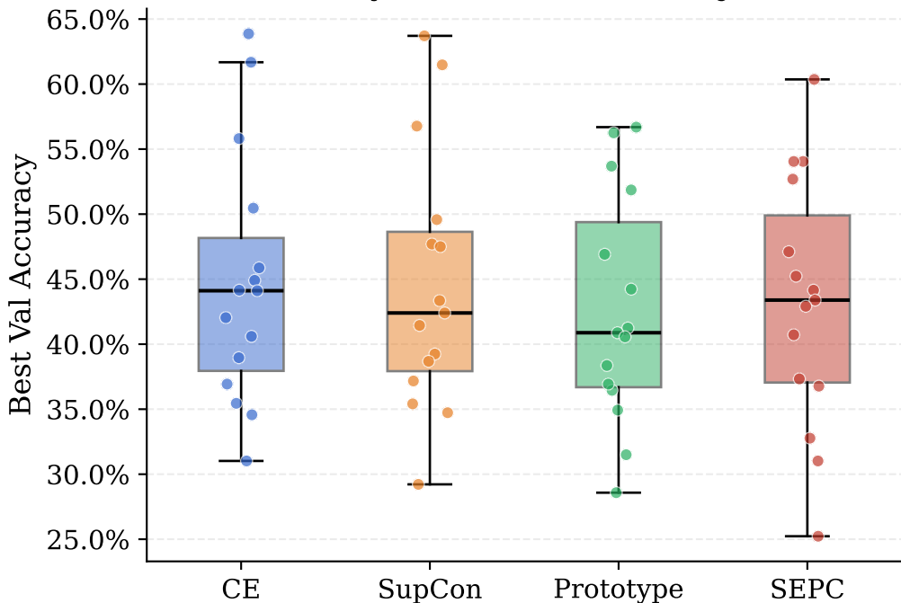
Accuracy Distribution (15 Subjects)
