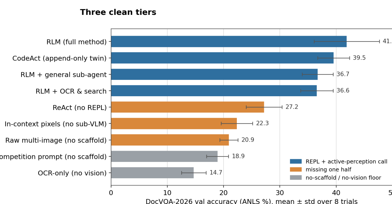
Fig. 2. Three clean tiers: REPL + perception (~36–42%), missing one half (21–27%), OCR-only floor (15%).
