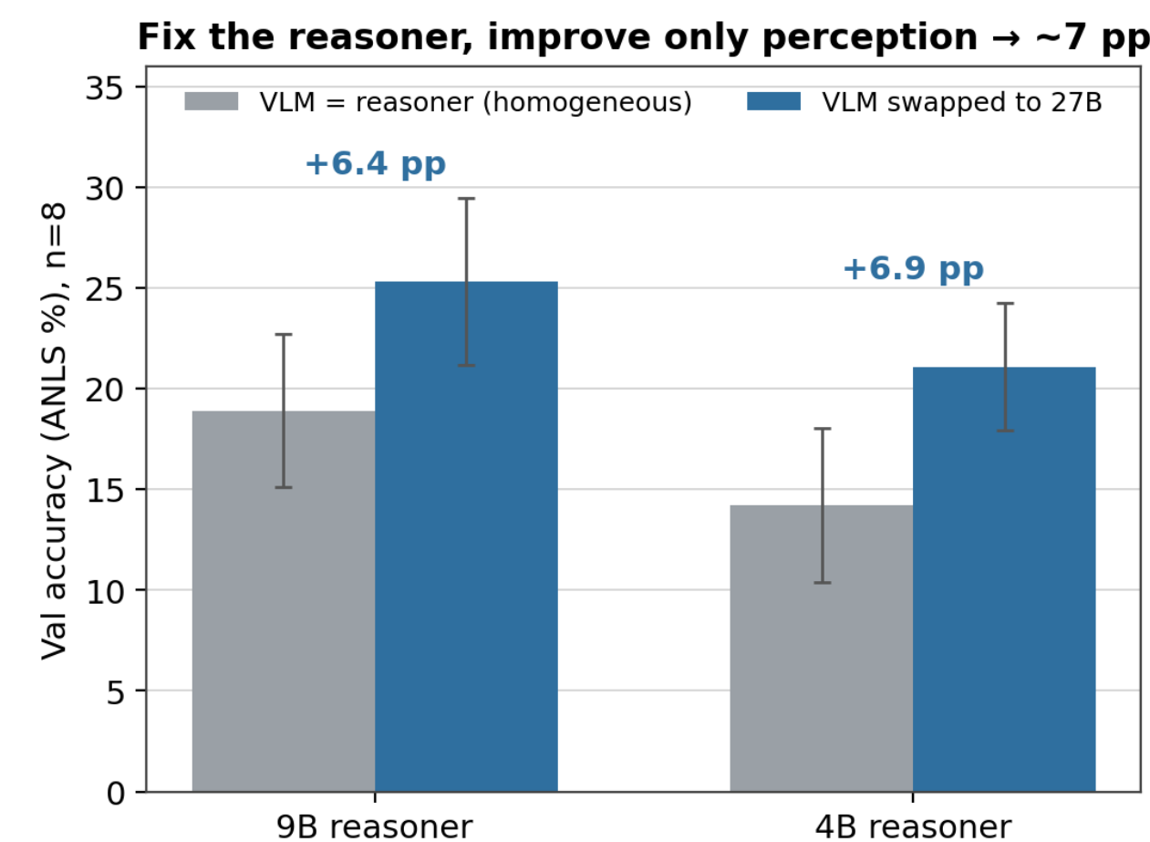
Fig. 3. Hold the reasoner fixed, feed its perception calls a stronger (27B) VLM: accuracy climbs ~7 pts at both reasoner sizes. Same brain, better eyes — a perception bottleneck.
