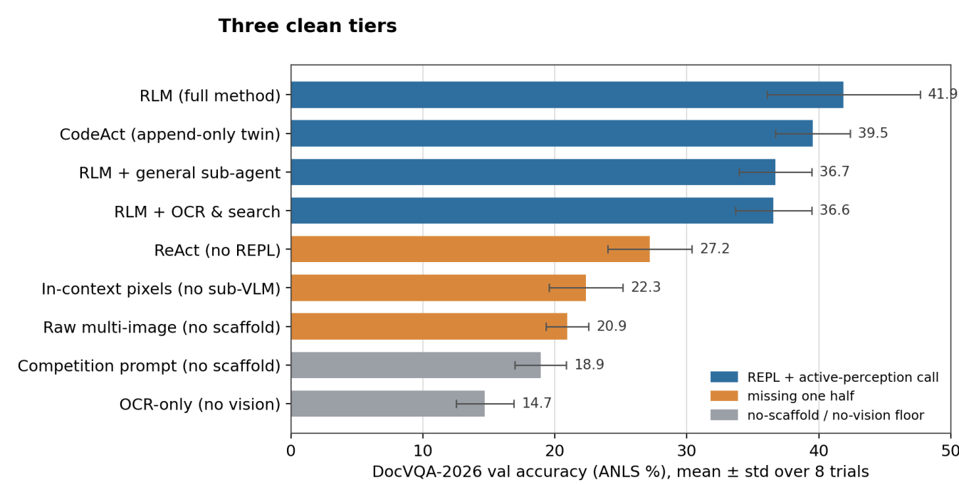
Fig. 2. Three clean tiers: REPL + perception (~36–42%), missing one half (21–27%), OCR-only floor (15%).
