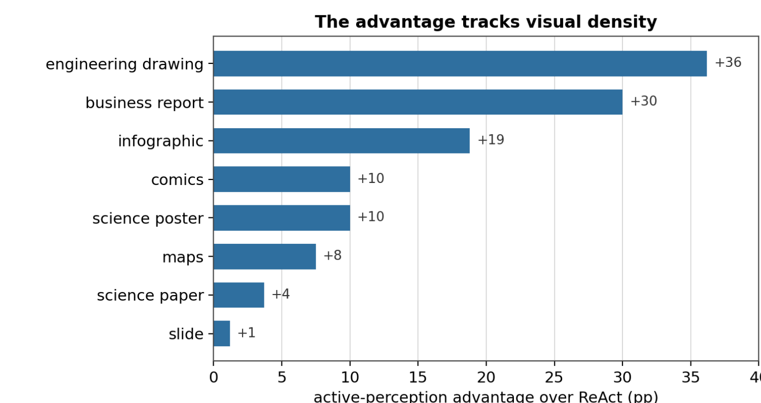
Fig. 4. Advantage over ReAct by category. Largest on dense, structured pages — engineering drawings (+36), business reports (+30), infographics (+19) — smallest on text-linear pages: science papers (+4), slides (+1).
